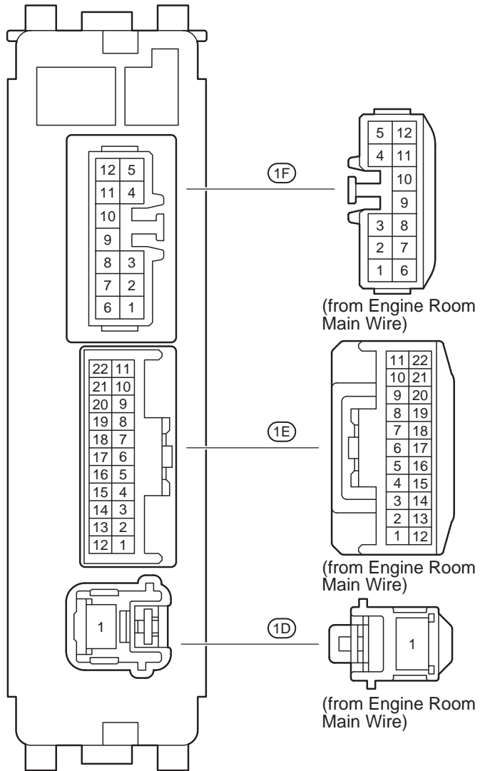
Back View
